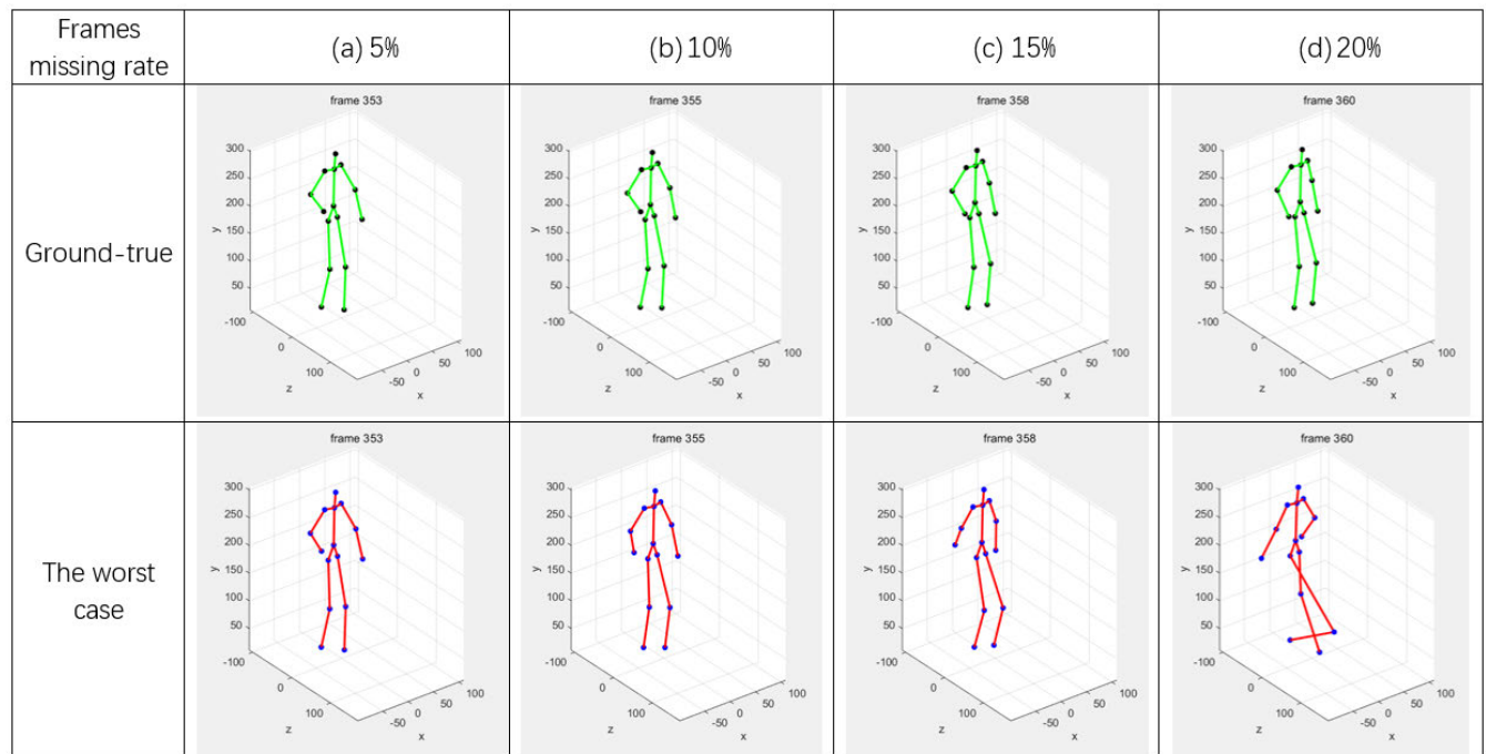
FIGURE 11. The worst cases of our method on 3D motion data with increasing whole frame missing rates.
