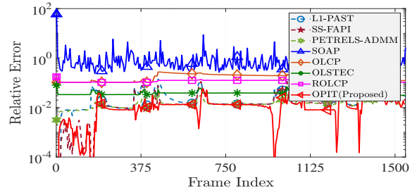
Fig. 3: Tracking ability of algorithms on the “Lobby” data.
