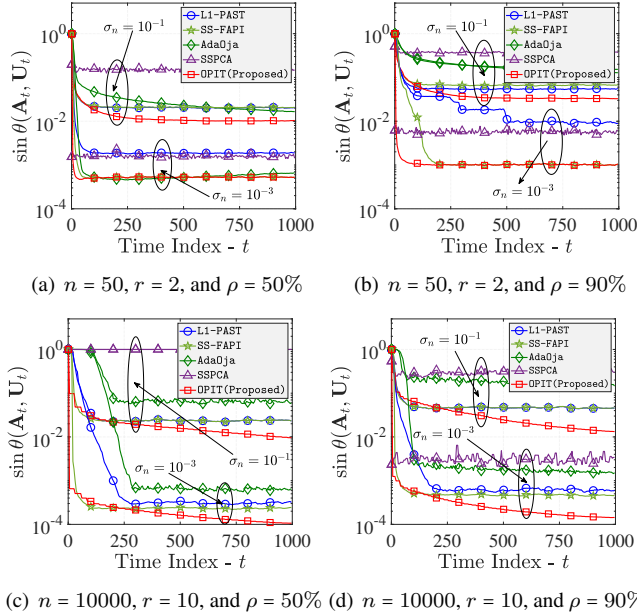
Fig. 1: Time-varying environments: data samples T = 1000 and time-varying factor \varepsilon = 10^{-3} .
