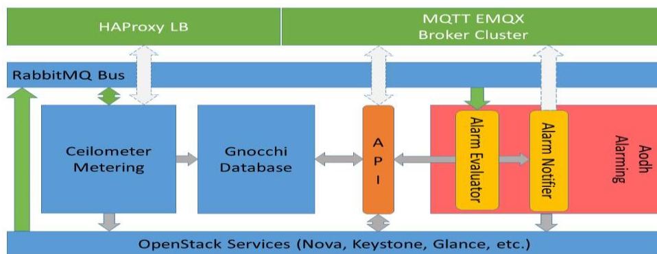
Figure 3. An implementation of Elastic MQTT Framework.
