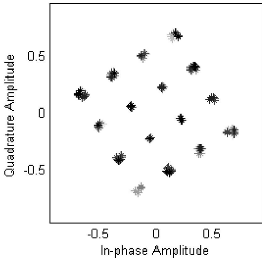
Fig. 4. A snap shot of the received 16-QAM constellation with multipath fading
