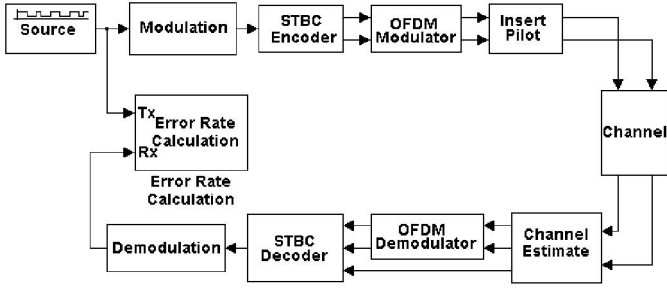
Fig. 1. STBC MIMO-OFDM system with pilot-aided method
