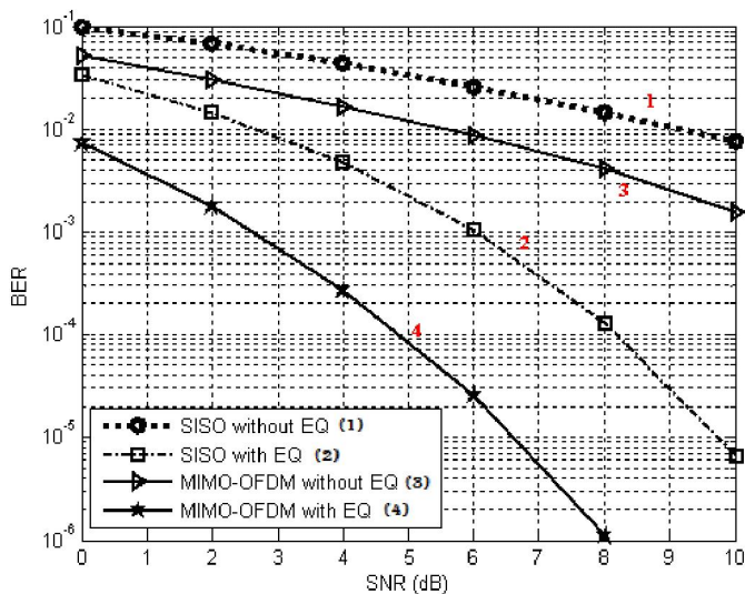
Fig. 6. The plot of BER vs SNR of four scenarios
