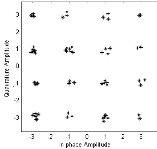
Fig. 5. Received 16-ary QAM constellation with AWGN plus multipath fading after the Equalizer block
