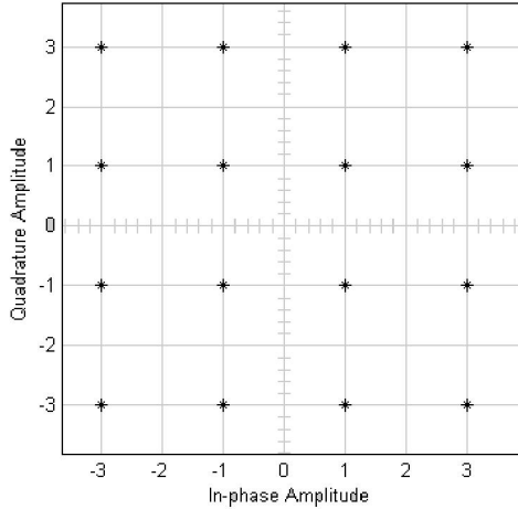
Fig. 3. Received 16-ary QAM constellation without any impairment
