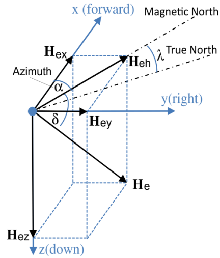
Fig. 2. Earth's magnetic field vector 0
