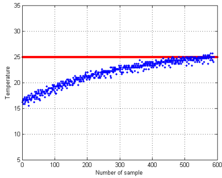
Fig. 16. Observation of temperature convergence using feed-forward compensation.
