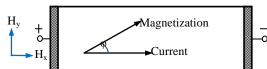
Fig. 3. Formation of \varphi in AMR sensor
