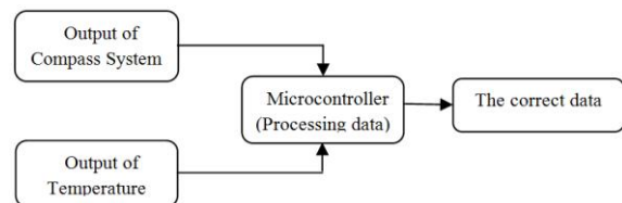
Fig. 6. Block diagram of the software compensated compass system
