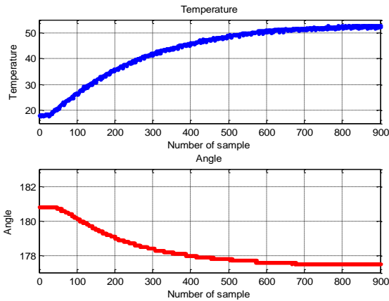
Fig. 12. Value of compass in 18-53°C of temperature range
