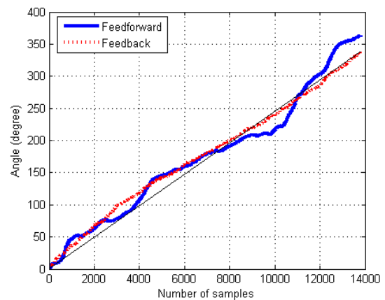
Fig. 20. The forward vs. feedback structures in compensating the angle values of the compass when it is placed on a turntable
