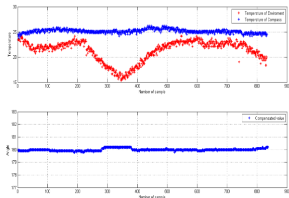
Fig. 15. Uncompensated vs. feedback compensated angles when the input temperature is fluctuating.
