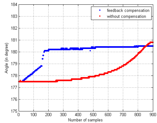
Fig. 14. Uncompensated vs. feedback compensated angles
