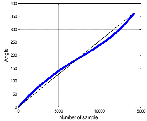
Fig. 19 The angle output of the compass sensor vs. the true angle while it was placed on a turntable at room temperature (i.e. 25°C)
