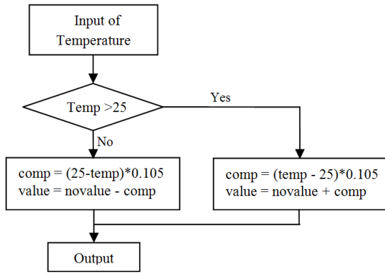
Fig. 7. Algorithm scheme of feed-forward compensation
