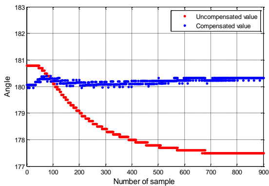
Fig. 13. Uncompensated vs. feed-forward compensated values of angles
