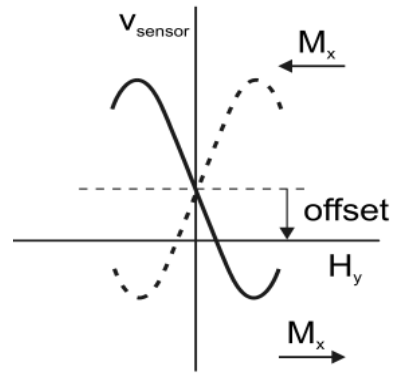
Fig. 5. The AMR sensor output after flipping of both polarities
