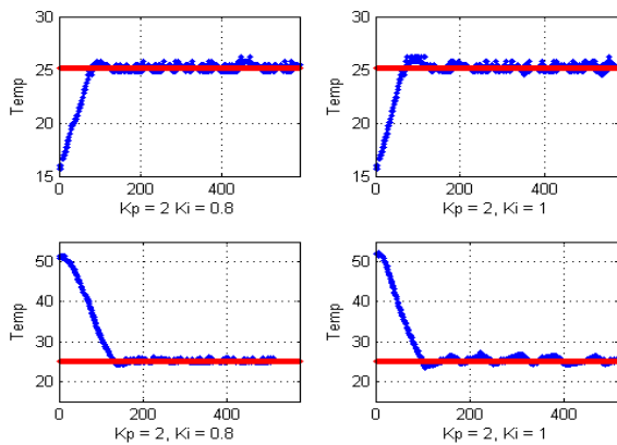
Fig. 18. The dependences of compensated outputs on the values of K_p , K_i
