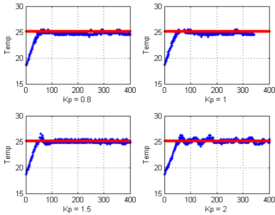
Fig. 17. The dependences of compensated outputs on the values of K_p .
