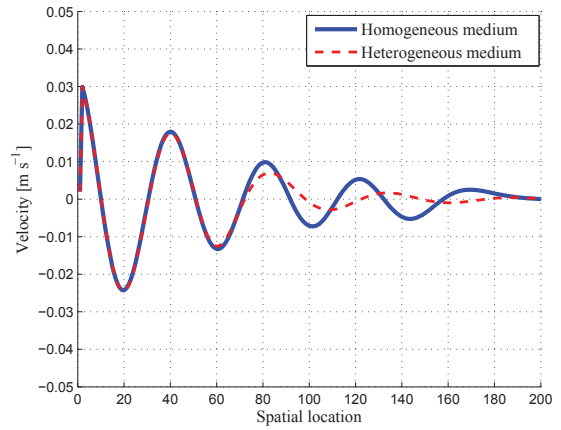
Fig. 4. The particle velocity in space, using FDTD model.
