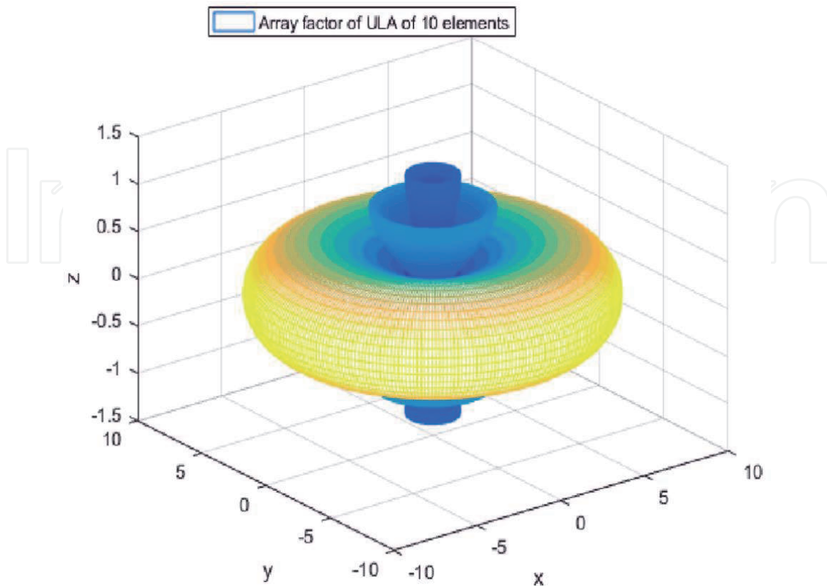
Figure 2. The array factor of ULA-analog-PA.
